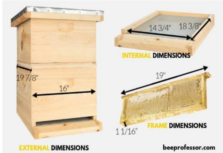
Fig 1. Standard 10 frame hive box for honeybee (https://beeprofessor.com/langstroth-hive-dimensions/)
