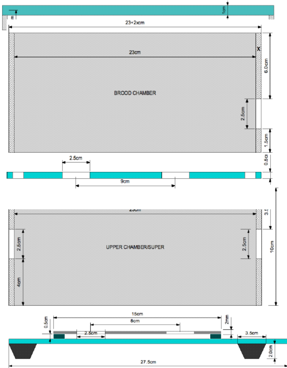
Fig 2. UPLB TPH Hive Box Dimension (UPLB Bee Program Intensive Beekeeping Course , 2022)
