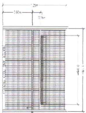
DETAILS OF STEEL GATE SCALE 1:20 (1/2" = 1'-0")
